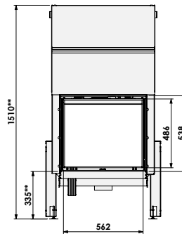
Evo-7 Compact 55-45
